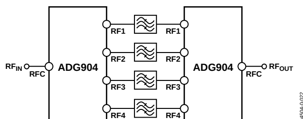
Figure 28. Filter Selection
